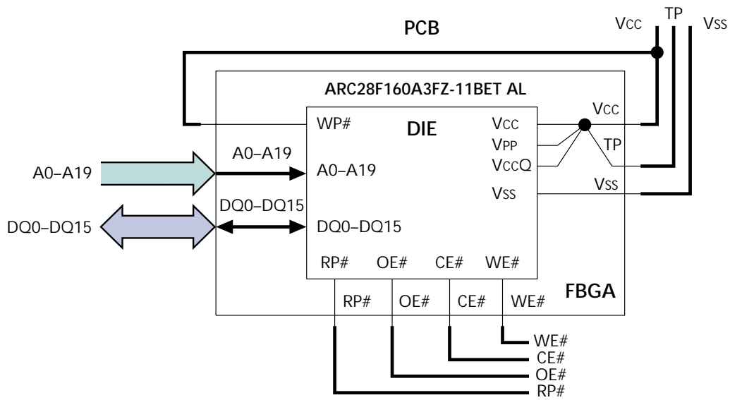
Figure 1 Diagram of Internal and External Connections
